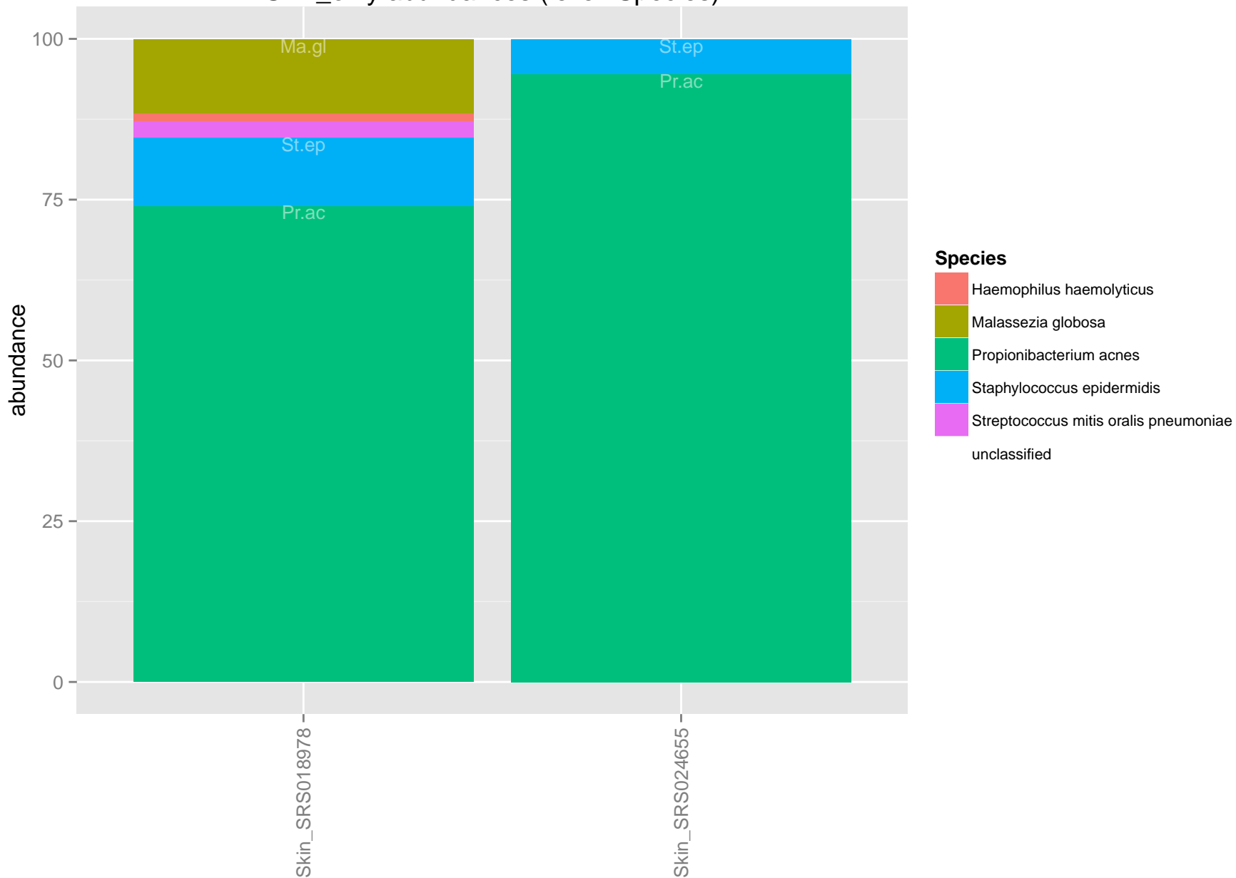
Skin_only abundances (level: Species)
