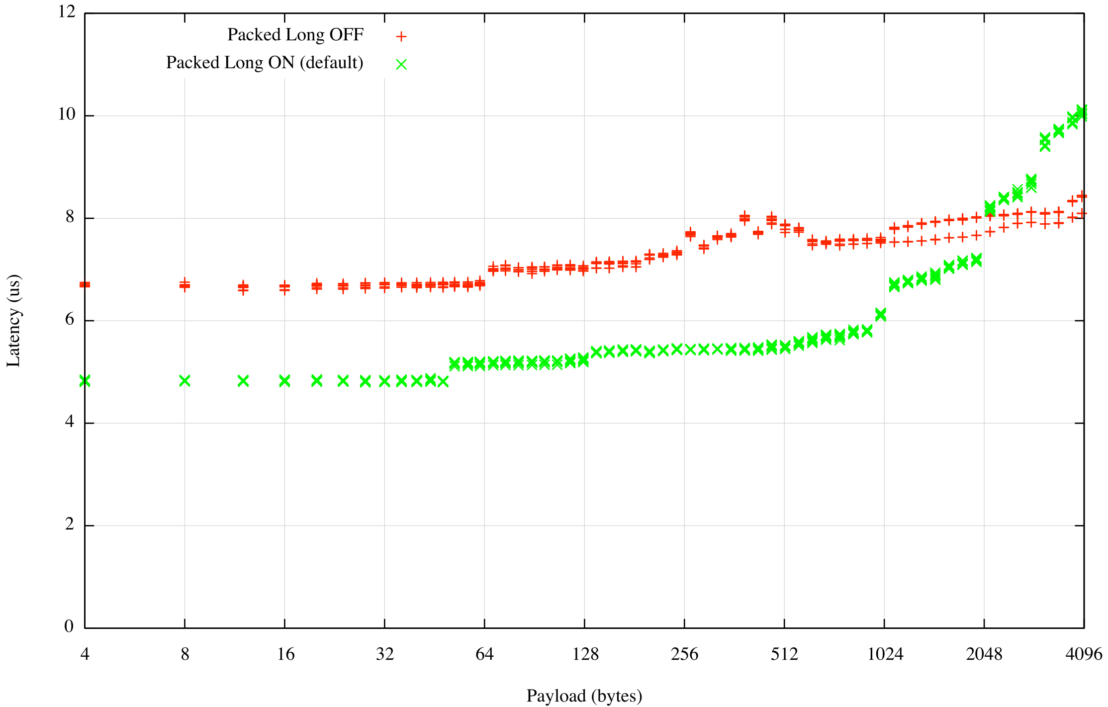
gex_AM_RequestLong0 ping-pong round-trip latency
